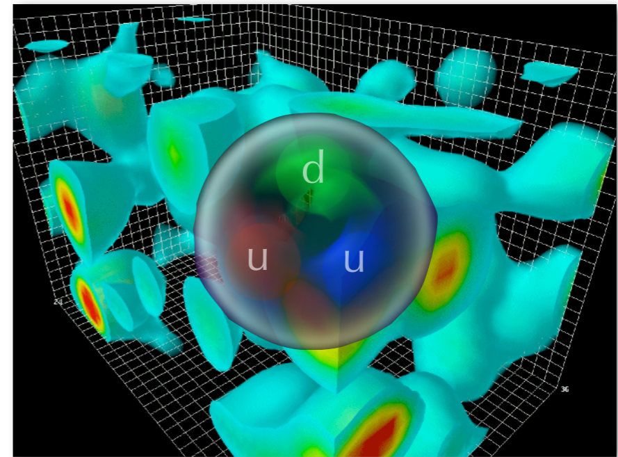
Lattice simulation, D. Leinweber (Adelaide)
